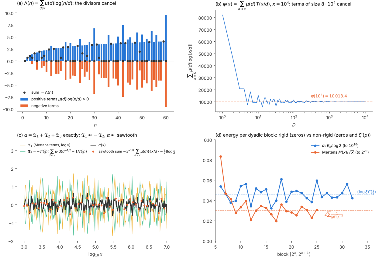
FIGURE 5. \Lambda = \mu * \log . (a) The divisor sum (20) for n \leq 60 : positive and negative terms, and their sum \Lambda(n) . (b) Partial sums of \psi(x) = \sum_{d \leq x} \mu(d) \log \lfloor x/d \rfloor! at x = 10^4 . (c) The exact decomposition of Proposition 25: \mathfrak{T}_1 and \mathfrak{T}_2 are mirror images, and \alpha follows the Möbius-weighted sawtooth (22) (dots). (d) Energy per dyadic block of \alpha (to 10^{10} ) and of the Mertens function M(x)/\sqrt{x} (to 2^{26} ), with their predicted means (\log \xi)''(\frac{1}{2}) and 2 \sum_{\gamma > 0} |\rho \zeta'(\rho)|^{-2} .
