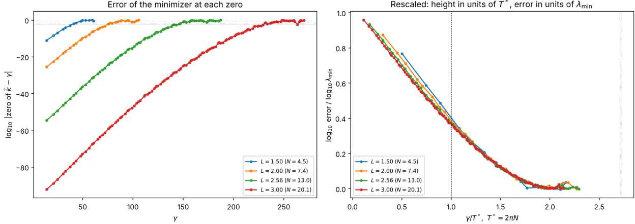
FIGURE 6. The minimizer of Weil's form in the windows N = 4.5, 7.4, 13, 20.1 [CE22]. Left: \log_{10} of the distance from each zero of \zeta to the nearest zero of the minimizer's transform. Right: the same data with the height in units of T^* = 2\pi N and the error in units of \lambda_{\min} ; dashed T^* , dotted eT^* .
