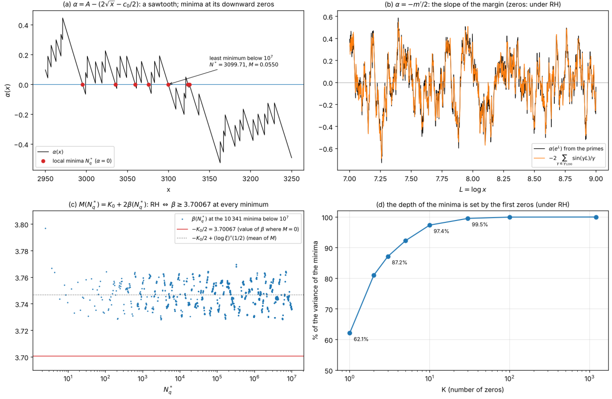
FIGURE 3. The minima read from the slope. (a) The sawtooth \alpha(x) on [2950, 3250] ; its downward zeros (red) are the local minima N_q^* , among them the least minimum below 10^7 . (b) \alpha(e^L) from the primes and -2 \sum_{\gamma \leq \gamma_{1200}} \sin(\gamma L)/\gamma from the zeros. (c) \beta(N_q^*) at the 10 341 minima below 10^7 ; the red line is M = 0 by (14). (d) Share of the variance of the minima reproduced by the first K zeros.
