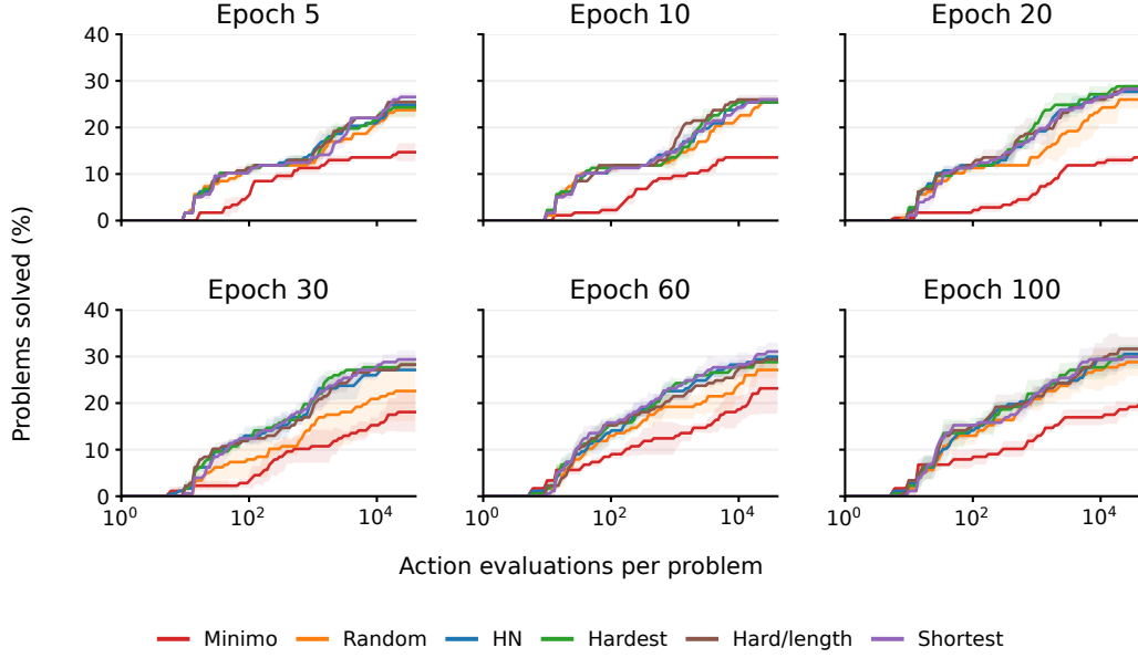
Figure 15: Abelian groups: best-first solve rate versus policy action evaluations per problem. Lines and bands show the three-seed mean \pm 1 sample SD.
