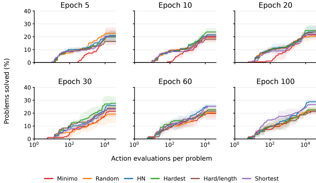
Figure 18: Abelian groups: rollout solve rate versus cumulative policy action evaluations per problem. Lines show three-seed means; shading shows \pm 1 sample SD.
