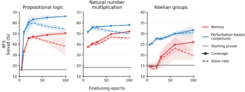
Figure 3: Training on samples from perturbation-based conjecturer yields higher BFS solve rates than training on Minimo-generated conjectures at every evaluated checkpoint in all three domains. Minimo’s solve rate declines after epoch 30 in logic and epoch 60 in groups, while its coverage continues to rise: later checkpoints solve new problems while losing some previously solved ones. Blue curves show the perturbation-based conjecturer with HN selection. Dashed curves show solve rate; solid curves with circles show coverage. Shading denotes \pm 1 sample SD across three seeds; solid gray lines show the starting prover’s performance.
