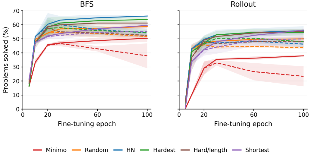
Figure 22: Propositional-logic learning curves for all methods: best-first search (left) and rollouts (right). Dashed lines show solve rate, solid lines show coverage, and shading shows \pm 1 sample SD.
