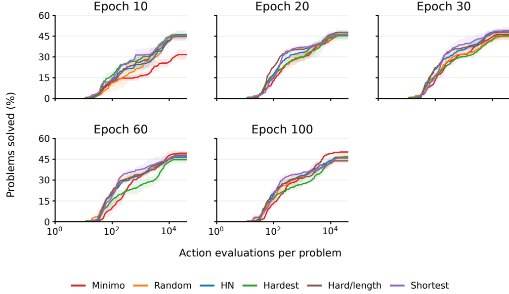
Figure 17: Arithmetic: rollout solve rate versus cumulative policy action evaluations per problem. Lines show three-seed means; shading shows \pm 1 sample SD.
