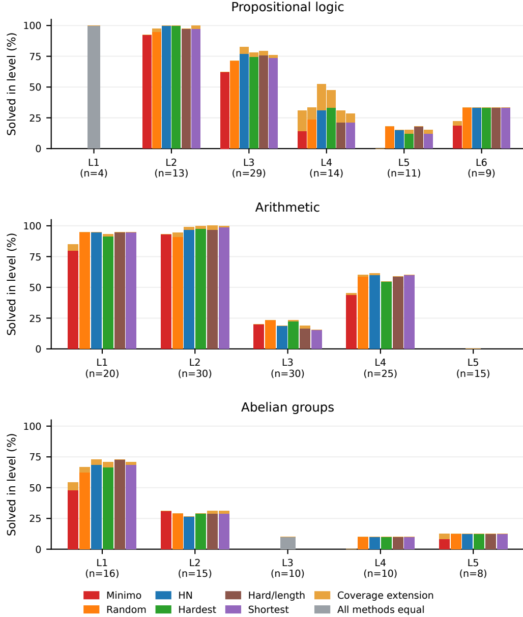
Figure 8: Level-wise best-first-search performance. Each panel show propositional logic, arithmetic, and abelian groups; n is the number of problems in each level. Colored bars show the maximum over checkpoints of the three-seed mean solve rate within that level. Gold extensions indicate coverage, computed by taking the union across checkpoints within each seed and then averaging. A gray bar represents all methods have the same performance; a missing bar has value zero.
