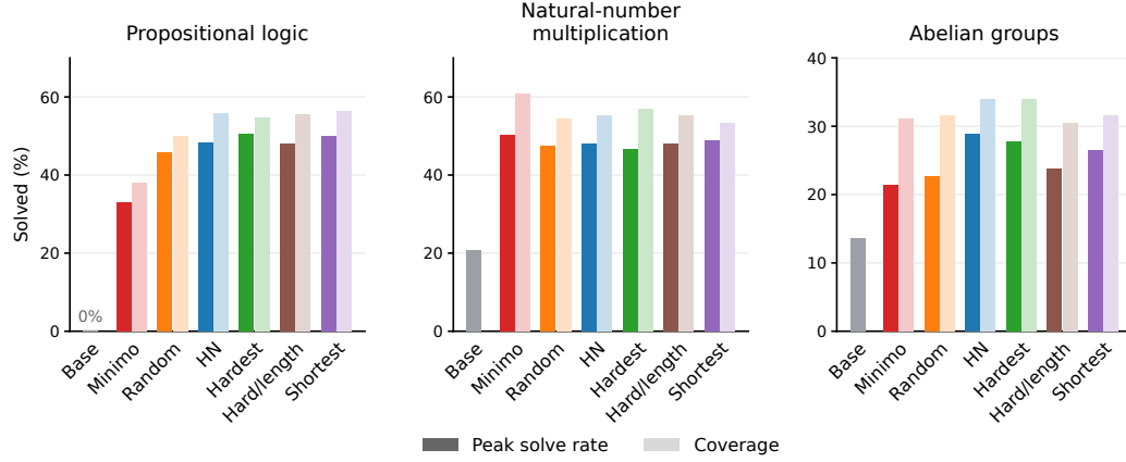
Figure 9: Overall rollout performance, including Base, Minimo, and all five perturbation selection methods. Each problem receives a greedy attempt followed by up to 16 sampled attempts. For trained methods, paired bars show peak solve rate (dark, left) and coverage (light, right): the maximum checkpoint-wise three-seed mean and mean within-seed coverage across checkpoints, respectively. Base is a single gray bar showing the starting prover’s solve rate.
