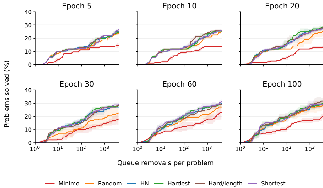
Figure 12: Abelian groups: best-first solve rate versus queue removals per problem, at all six evaluated checkpoints. Lines show three-seed means and shading shows \pm 1 sample SD.
