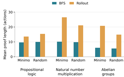
Figure 7: Rollout proofs are about 1.5\times as long as BFS proofs in logic and 2\text{--}3\times as long in arithmetic and groups. Bars show mean lengths on matched solved problems (Appendix I.3).
