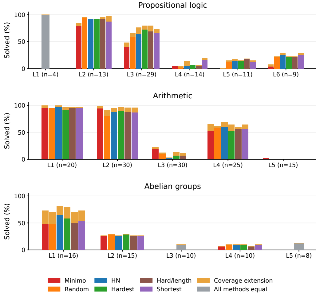
Figure 26: Level-wise rollout performance. Colored bars show the peak checkpoint-wise three-seed mean within each level; gold bars indicate mean within-seed coverage.
