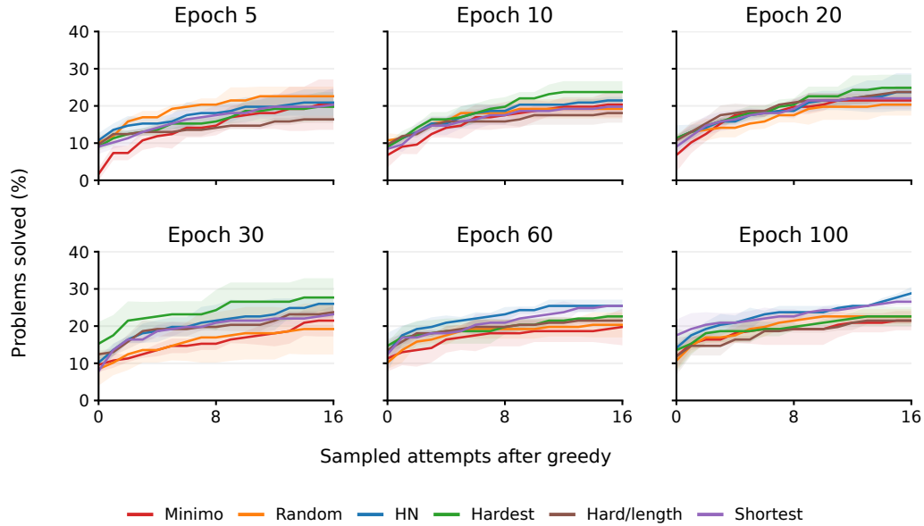
Figure 21: Abelian groups: solve rate after a greedy attempt plus up to k sampled attempts. Lines show three-seed means; shading shows \pm 1 sample SD.
