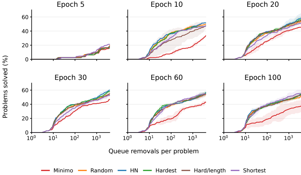
Figure 10: Propositional logic: best-first solve rate versus queue removals per problem, at all six evaluated checkpoints. Lines show three-seed means and shading shows \pm 1 sample SD.
