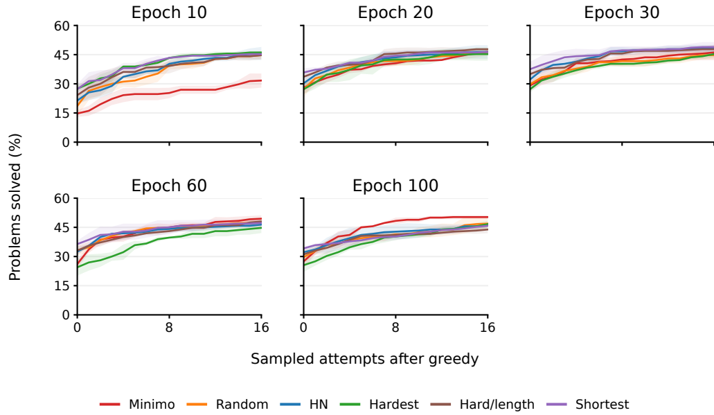
Figure 20: Arithmetic: solve rate after a greedy attempt plus up to k sampled attempts. Lines show three-seed means; shading shows \pm 1 sample SD.
