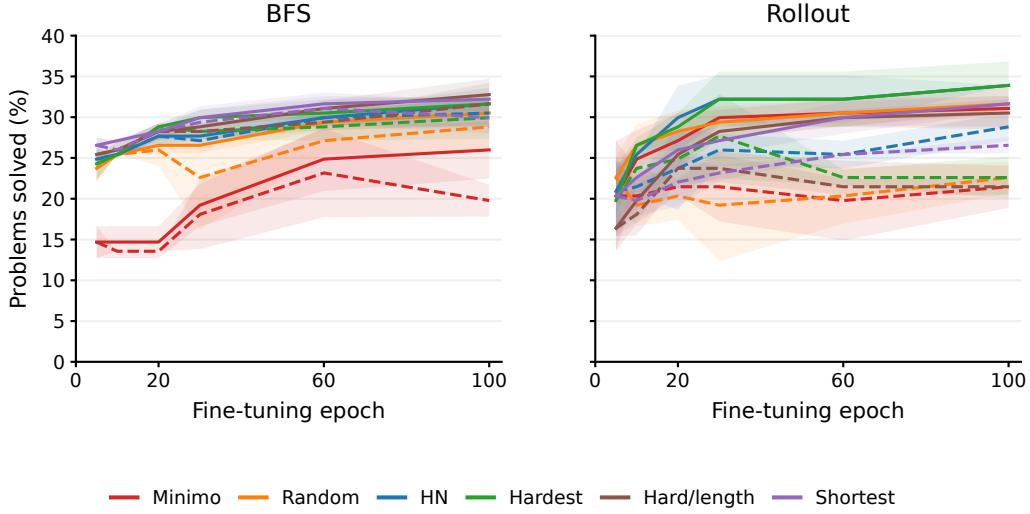
Figure 24: Abelian-group learning curves for all methods: best-first search (left) and rollouts (right). Dashed lines show solve rate, solid lines show coverage, and shading shows \pm 1 sample SD.
