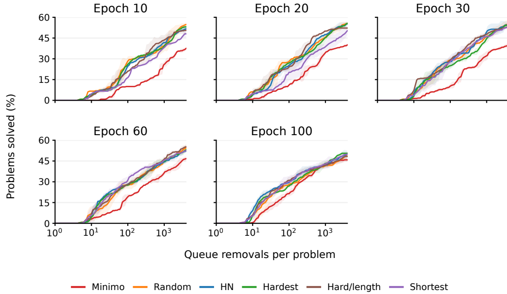
Figure 11: Arithmetic: best-first solve rate versus queue removals per problem, at all five evaluated checkpoints. Lines show three-seed means and shading shows \pm 1 sample SD.
