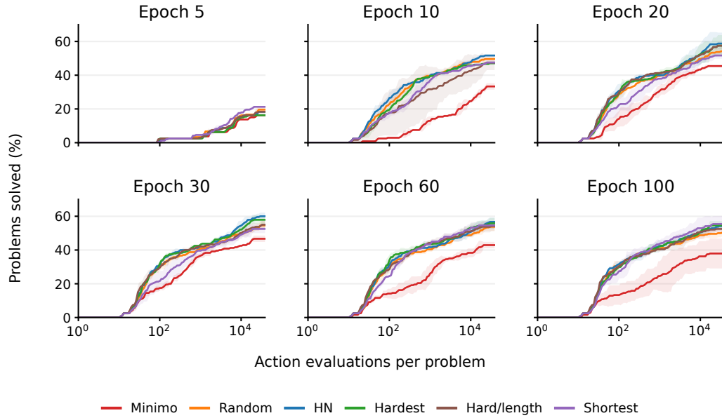
Figure 13: Propositional logic: best-first solve rate versus policy action evaluations per problem. Lines and bands show the three-seed mean \pm 1 sample SD.
