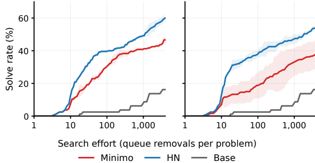
Figure 6: BFS solve rate versus search effort in propositional logic at epochs 30 (left) and 100 (right). Minimo and HN show three-seed means with \pm 1 sample SD shading; Base (solid gray) is the starting prover baseline.
