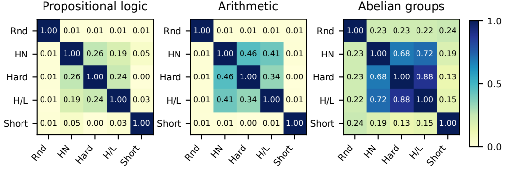
Figure 28: Mean within-seed Jaccard overlap of selected conjecture sets. Rnd denotes Random, Hard denotes Hardest, H/L denotes Hard/length, and Short denotes Shortest.
