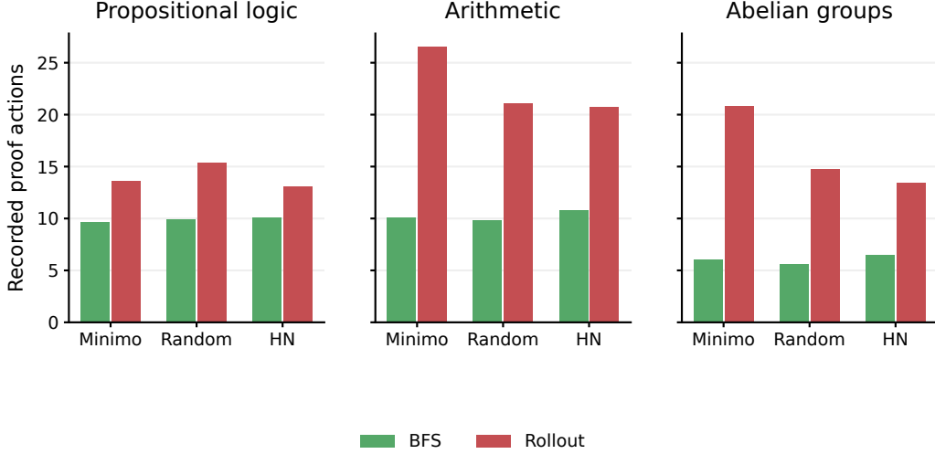
Figure 27: Mean returned proof lengths for BFS and rollout on problems solved by all three displayed methods under both searches, matched within each seed and checkpoint.
