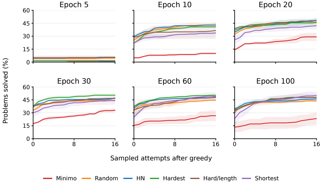
Figure 19: Propositional logic: solve rate after a greedy attempt plus up to k sampled attempts. Lines show three-seed means; shading shows \pm 1 sample SD.
