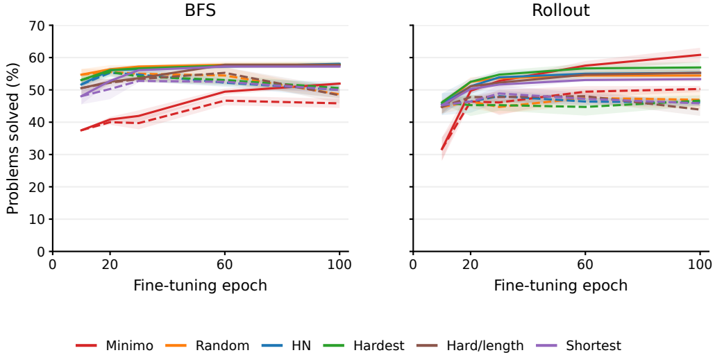
Figure 23: Arithmetic learning curves for all methods: best-first search (left) and rollouts (right). Dashed lines show solve rate, solid lines show coverage, and shading shows \pm 1 sample SD.
