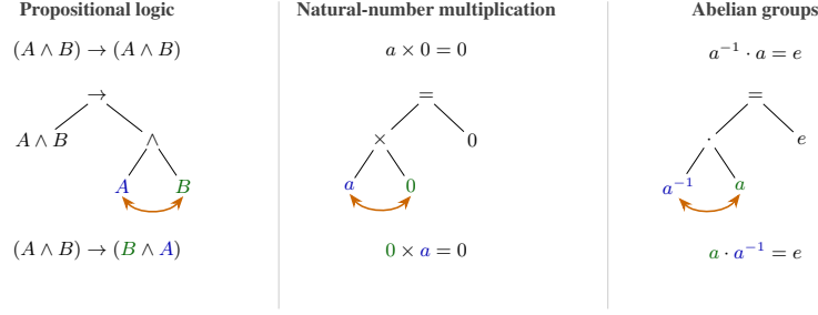
Figure 2: One perturbation across three domains: swapping two arguments in a statement’s abstract syntax tree yields a new candidate statement. Colors track the swapped subterms. These are simple syntactic edits that need not preserve truth or increase difficulty; Appendix A lists all perturbations we did per domain.
