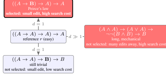
Figure 5: Hard Neighbours: small structural changes can produce large jumps in proof-search difficulty. Red marks costly statements; the thick border marks the HN selection.
