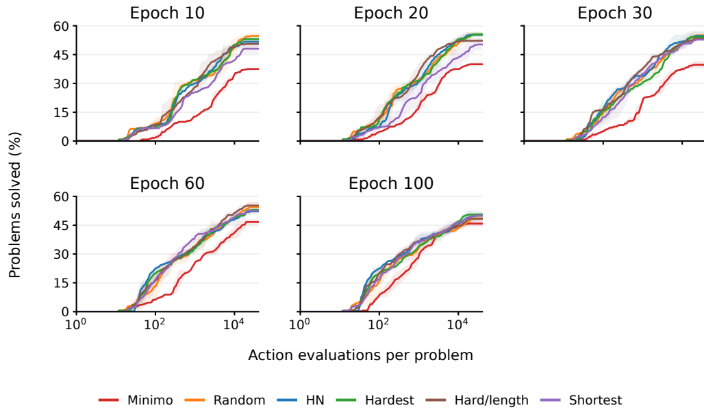
Figure 14: Arithmetic: best-first solve rate versus policy action evaluations per problem. Lines and bands show the three-seed mean \pm 1 sample SD.
