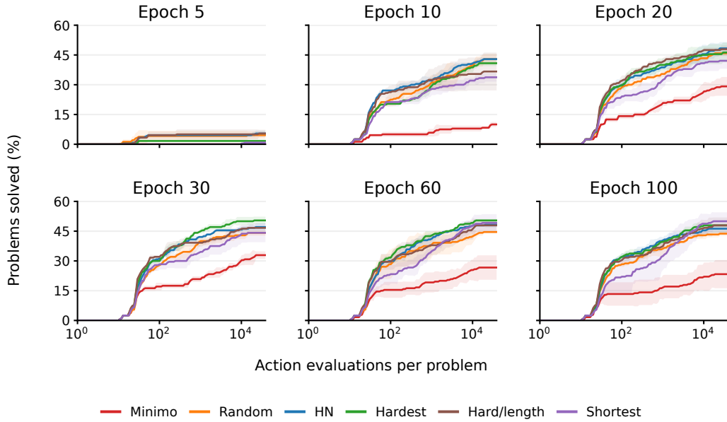
Figure 16: Propositional logic: rollout solve rate versus cumulative policy action evaluations per problem. Lines show three-seed means; shading shows \pm 1 sample SD.
