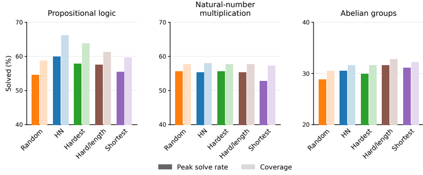
Figure 4: Selection gains vary by domain under best-first search at a 4,000-removal budget. Selection helps most in logic, where HN improves on Random by about 5 percentage points in peak solve rate and 8 points in coverage. In groups, Hard/length leads, exceeding Random’s peak solve rate by about 3 points; in natural-number multiplication, no method exceeds Random’s peak. Each pair shows peak solve rate (dark, left) and coverage (light, right) (Section 6.1)
