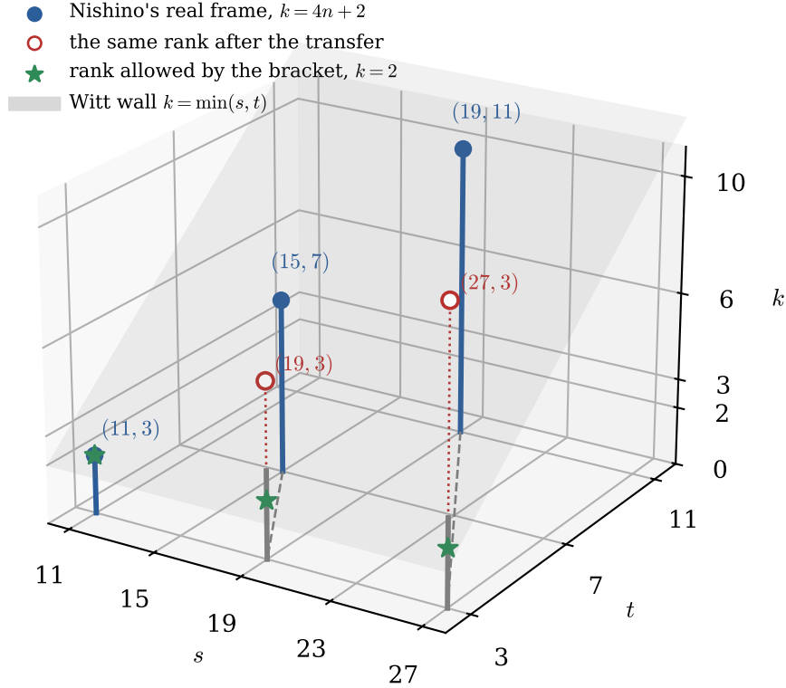
FIGURE 8. The transfer in the space of signatures and ranks (s, t, k) . Blue: Nishino's real frames of rank 4n + 2 in (11 + 4n) + (3 + 4n) for n = 0, 1, 2 , all below the wall k = \min(s, t) (grey). Dashed: moving 4n times into space. Red circles: the same ranks in (11 + 8n) + 3 , above the wall, since a real frame there has at most three null vectors. Green stars: the rank k = 2 , the only one compatible with the translation bracket; at n = 0 it is Sezgin's theory in 11 + 3 .
