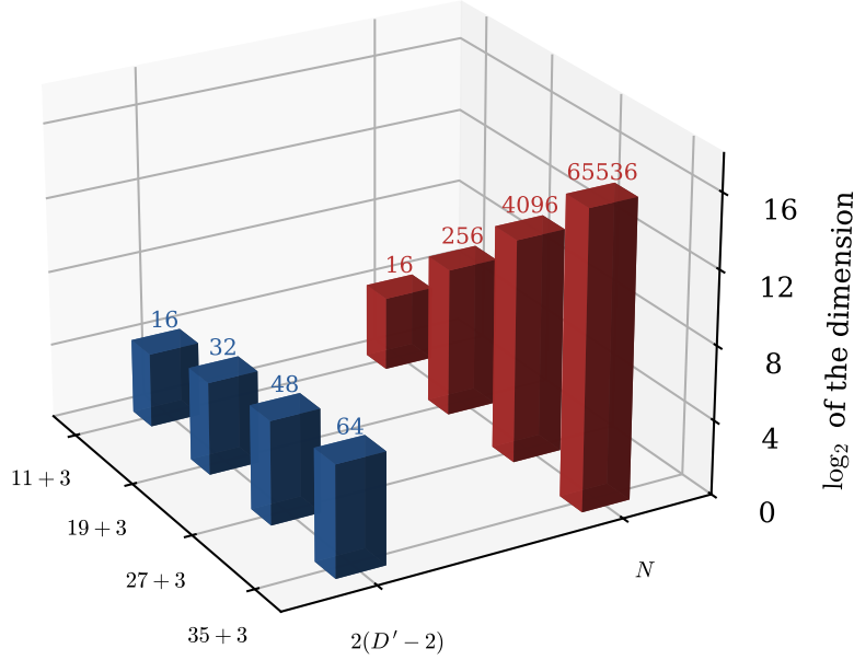
FIGURE 9. At rank two in (11 + 8n) + 3 , the dimension N = 2^{4+4n} of the residual Weyl module (red) against the dimension 2(D' - 2) = 16 + 16n that absorption of the cubic terms requires by Theorem 3.3 (blue), on a logarithmic scale. They agree only for 11 + 3 , Sezgin’s theory.
