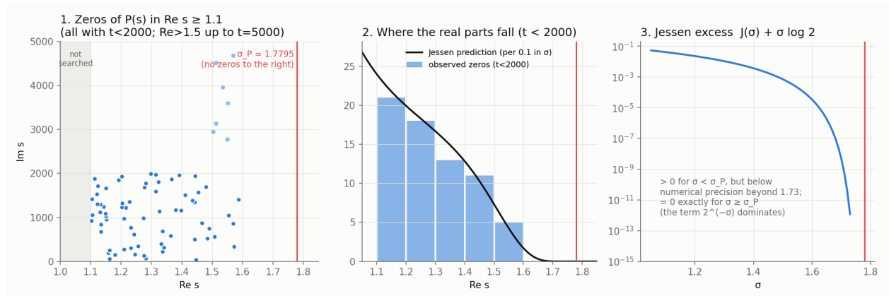
FIGURE 2. Left: zeros of P with \text{Re } s \geq 1.1 (all below height 2000; those with \text{Re } s > 1.5 up to height 5000; counts certified, locations floating point) and the edge \sigma_P . Centre: distribution of real parts below height 2000 against the Jessen prediction TJ''(\sigma)/2\pi . Right: the excess J(\sigma) + \sigma \log 2 .
