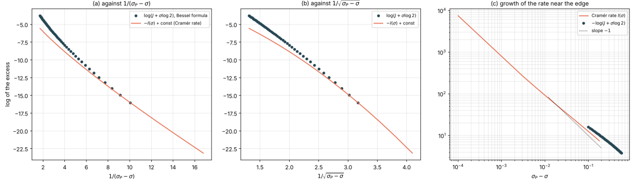
FIGURE 1. The Jessen excess near the edge (numerical, not certified). (a), (b): \log(J(\sigma) + \sigma \log 2) from the Bessel formula, for 1.2 \leq \sigma \leq 1.68 (above the error floor), against 1/(\sigma_P - \sigma) and 1/\sqrt{\sigma_P - \sigma} , with -I(\sigma) shifted by a constant, I the Cramér rate of Section 3. (c): I(\sigma) and -\log(J + \sigma \log 2) against \sigma_P - \sigma on logarithmic axes.
