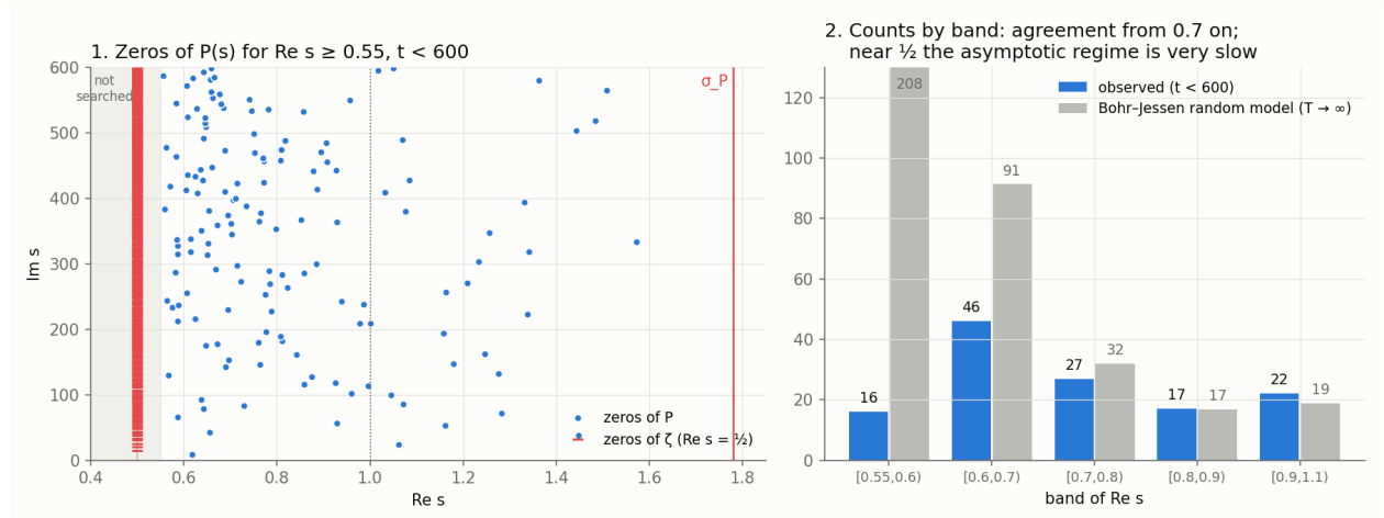
FIGURE 3. Left: zeros of P with \operatorname{Re} s \geq 0.55 below height 600 (branch of Proposition 5.1(b); floating point), with the zeros of \zeta on the critical line. Right: counts by band of \operatorname{Re} s against the asymptotic Bohr–Jessen prediction, which is not proved to apply inside the critical strip.
