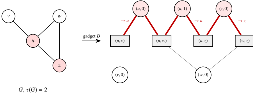
Figure 5: The edge-dominating-set gadget of c_{10} . Left: a graph G in which u has neighbours v, w, z (adjacency order) and w, z are adjacent. Right: its gadget D . Every edge of G is an edge-node (grey box); every vertex receives incidence nodes (circles) that thread its edge-nodes into a path, e.g. (u, v) - (u, 0) - (u, w) - (u, 1) - (u, z) for u , while v , of degree 1, has the single node (v, 0) . The incidence index k in (u, k) is a position on the path of u , never a neighbour. The thick red edges are all the path edges of the vertices labelled 1, u and z (shaded): they form an edge dominating set of D , since every gadget edge shares an endpoint with one of them, and they decode to the cover \{u, z\} . Its weight is 2K^* + 1 : one unit K^* per vertex, and an overlap of 1 because the edge uz has both endpoints in the cover. Every minimum cover of G ( \{u, z\} or \{u, w\} ) has this weight, and no other labelling is lighter.
