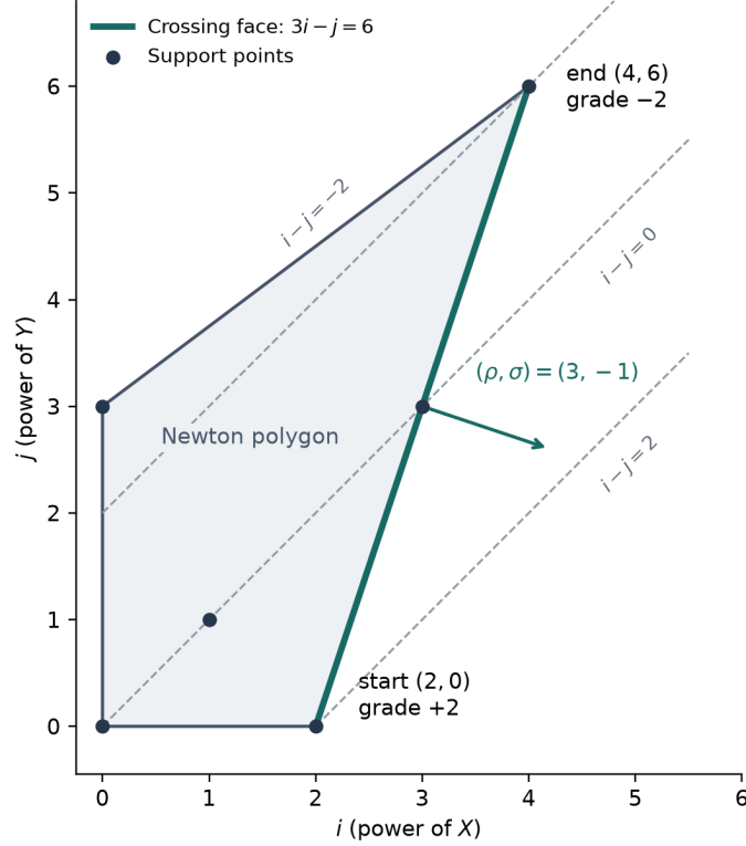
Figure 1: An illustrative support with a strict crossing in direction (3, -1) . The face lies on 3i - j = 6 ; its starting point has grade 2 and its ending point has grade -2 . Dashed lines have constant grade i - j . The figure illustrates the definitions and makes no claim about the existence of a Weyl mate.
