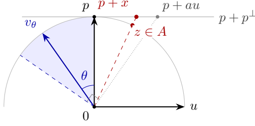
FIGURE 1. A two-dimensional section through p and u . Central projection follows the ray through z to p + x . When \langle x, u \rangle \leq a , directions with 0 \leq \theta < \theta_a lie in the positive polar. The sector's limiting boundary ray is orthogonal to p + au .
