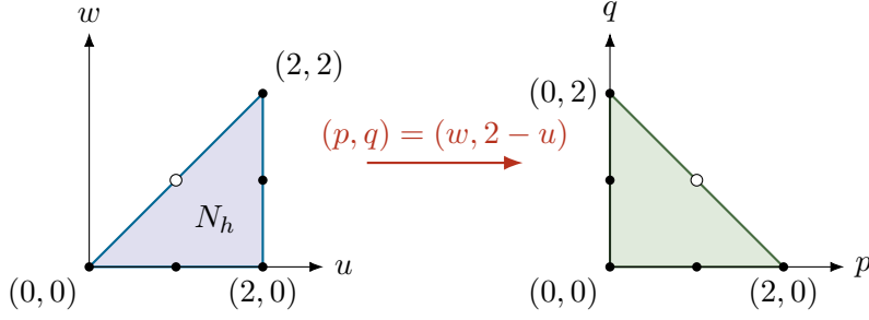
FIGURE 1. The carrier for (b, c) = (2, 2) and h = (-2, 2) and its image in pointed coordinates. The vertices (0, 0), (2, 0), (2, 2) map respectively to (0, 2), (0, 0), (2, 0) . Filled points have nonzero weights; the open point (1, 1) has weight zero in both coordinate systems. This is the specific affine example of Section 7.2.
